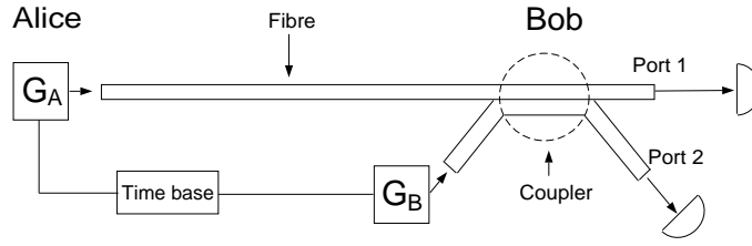
Figure 1 The schematic diagram of the quantum cryptosystem using an optical coupler. Alice's (or sender's) signal generator is labeled by G_A ; Bob's (or receiver's) is labeled by G_B .
