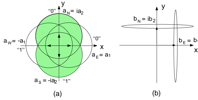
Figure 2 On planes of quadrature-phase amplitudes, (a) shows Alice's encoding strategy based on four nonorthogonal coherent states; (b) shows Bob's tap-fibre modes using squeezed light. Uncertainty of a state is represented by error ellipses for squeezed states and by error circles for coherent states.
